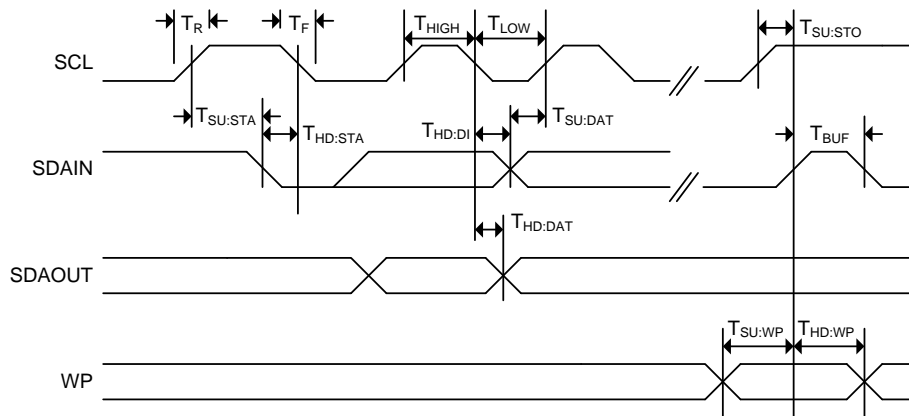
Figure 5.6. Bus Timing
