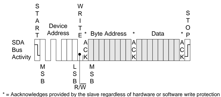
Figure 6.1 Byte Write
