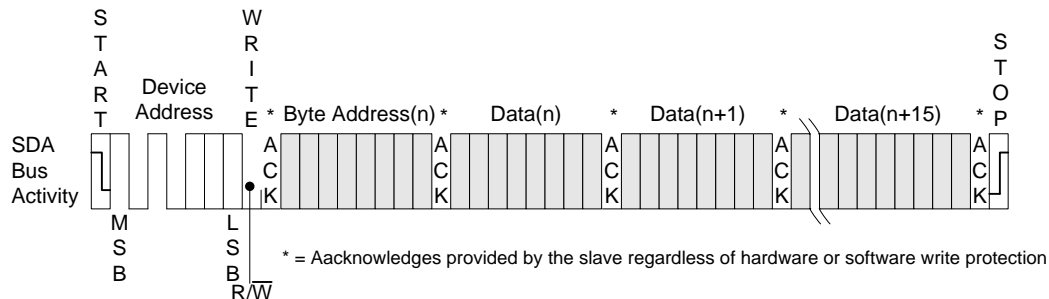
Figure 6.2 Page Write
