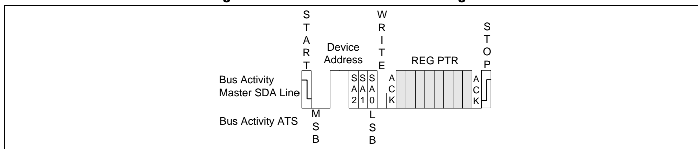
Figure 7.2 I 2 C Bus Write to Pointer Register
