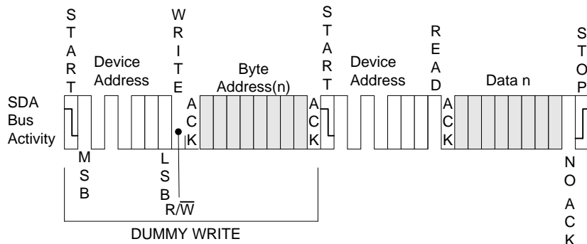
Figure 6.3 Random Address Read
