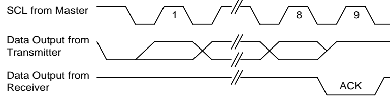
Figure 5.5. Output Acknowledge
