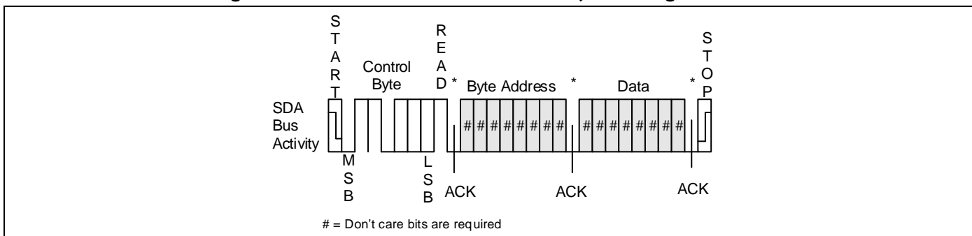
Figure 6.7 Read Write Protection Status; Read Page Address
