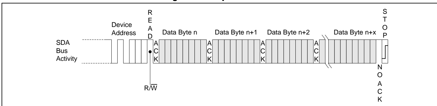
Figure 6.5 Sequential Read
