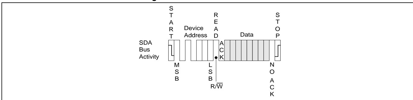
Figure 6.4 Current Address Read
