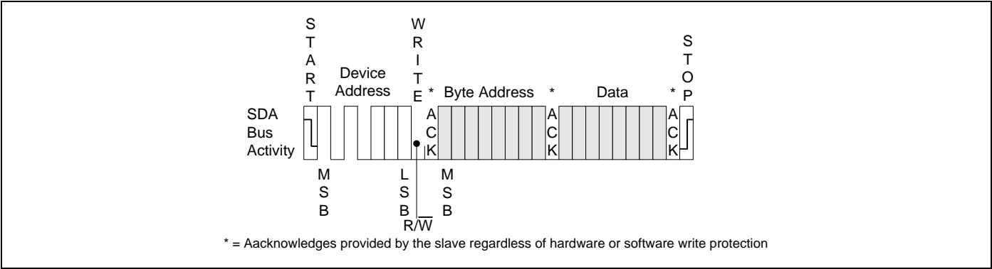
Figure 6.1 Byte Write
