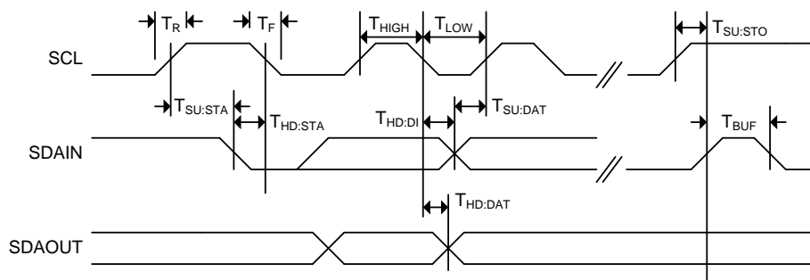
Figure 5.6. Bus Timing
